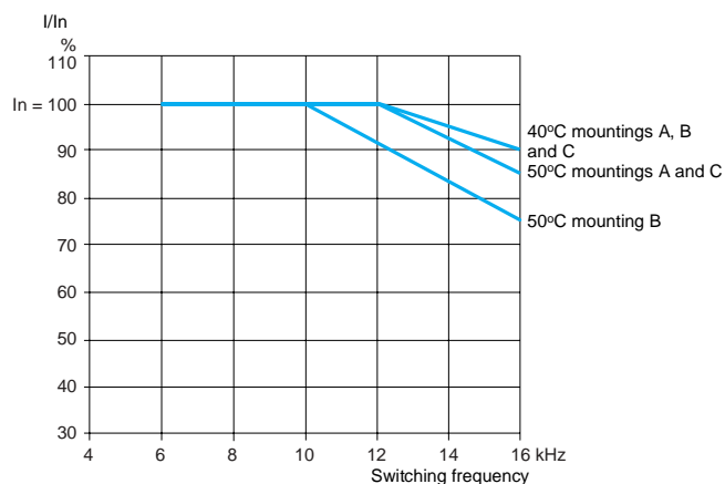
ATV 21HU40N4
